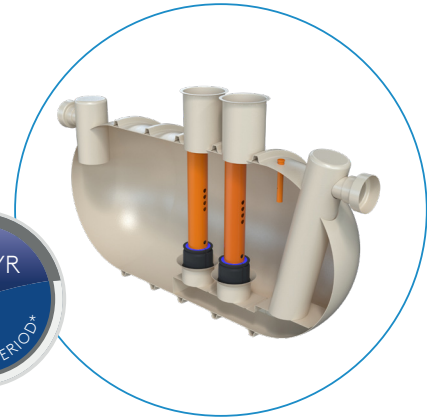
AquaTreat Full Retention GRP Surface Water Treatment Separator
