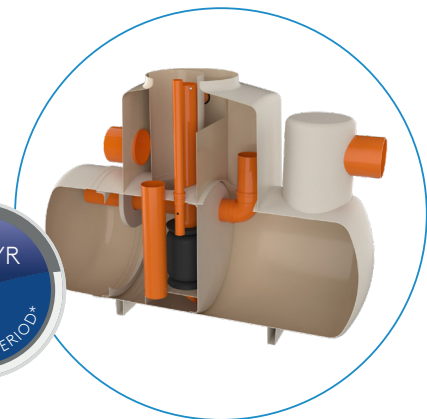
AquaTreat Bypass GRP Surface Water Treatment Separator
